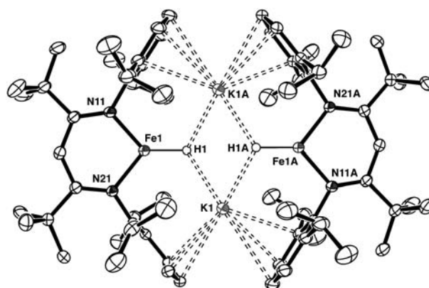
Figure 1. Thermal ellipsoid plot of [(KL tBu,iPr2 FeH) 2 ]. Ellipsoids are set at 50% probability. The two monomeric fragments are related by an inversion center. Selected bond lengths [Å] and angles [°]: Fe–N 1.914(1), 1.916(1), Fe–H 1.62(2); N–Fe–N 99.26(6), N–Fe–H 131.7(9), 129.0(8).
